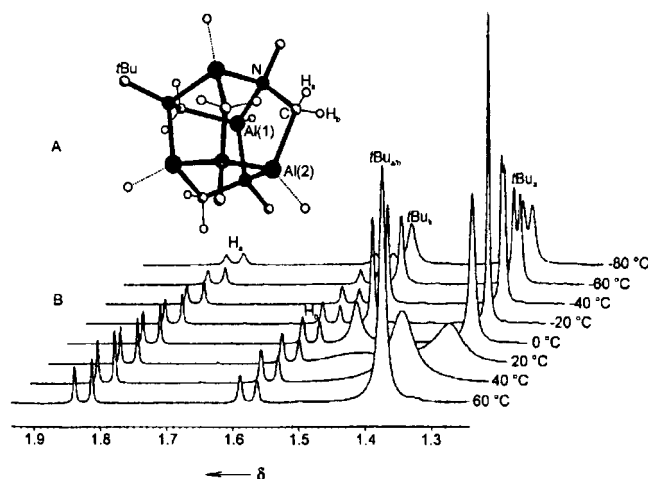
Figure 1. A) Molecular structure of 1 ( t\text{Bu} groups are represented by C atoms). Selected bond lengths [Å] and angles [°]: Al(1)–N(1) 1.968(2), Al(1)–N(2) 1.9693(19), Al(1)–C(4) 1.992(2), N(1)–C(1) 1.529(3); N(1)–Al(1)–N(2) 104.44(8), N(1)–Al(1)–C(4) 107.09(9), N(2)–Al(1)–C(4) 98.60(9), C(1)–N(1)–Al(1) 105.42(13), C(1)–N(1)–Al(2) 106.33(13), Al(1)–N(1)–Al(2) 102.49(8), N(1)–C(1)–Al(3) 109.95(14), N(2)–C(2)–Al(2) 110.07(14). B) Variable-temperature ^1\text{H} NMR spectra of 1 in [\text{D}_8]\text{toluene} .
